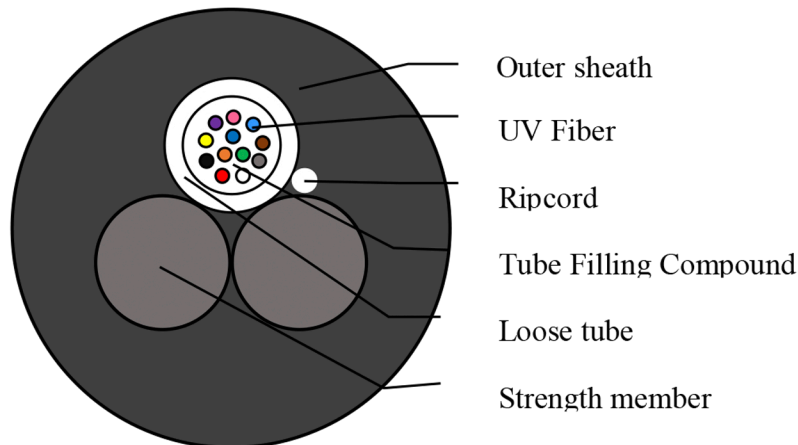
Figure. Cable Cross-Section (A-end)
