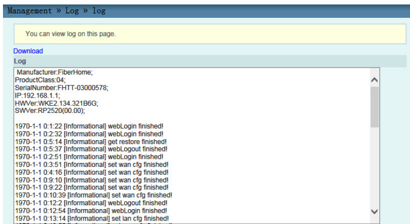
Figure 4.29 Log
