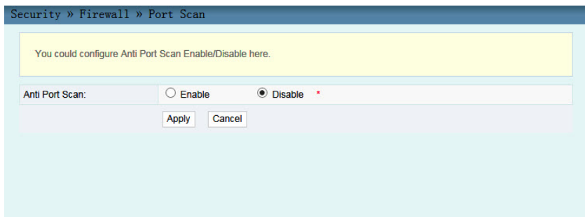
Figure 4.14 Anti-port Scan
