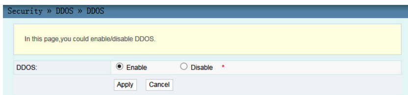
Figure 4.17 DDOS
