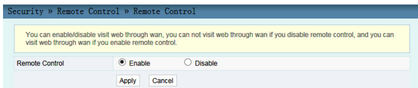
Figure 4.16 Remote Control
