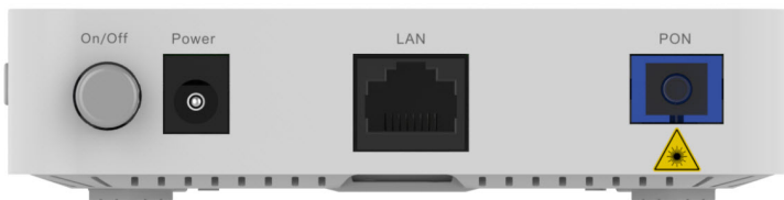
Figure 3.2 Rear Panel of the AN5506-01-A
