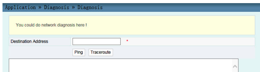
Figure 4.22 Network Diagnosis
