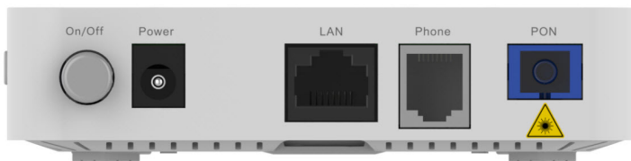
Figure 3.5 Rear Panel of the AN5506-01-B
