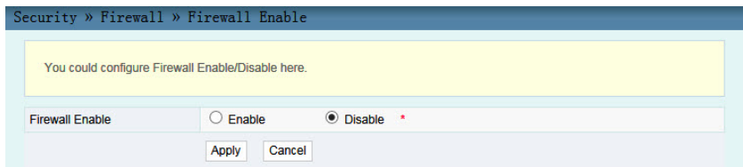
Figure 4.11 Firewall Enabling
